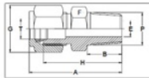
Male Stainless steel Compression Connectors
